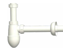
9B632-010-I011 Drain pipe for basin Pipe diameter: Ø32mm Distance between wall & inlet: 240mm Material: pp
