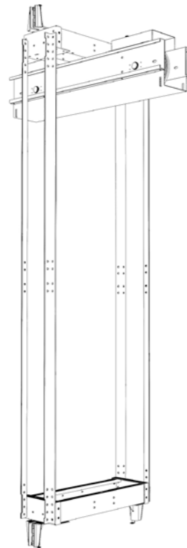
2/1 KARKAS - S21 2/1 CARCASS - S21
