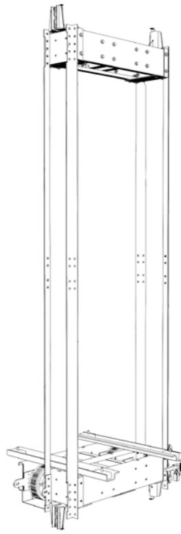
2/1 KARKAS - S30 2/1 CARCASS - S30
