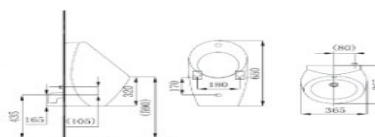
J13043-1/31Z-1 Wall-hung sensor urinal
